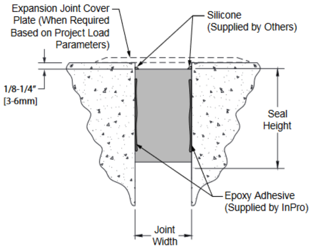
995H3 Floor/Floor Uncoated (995H3-250 UC)
