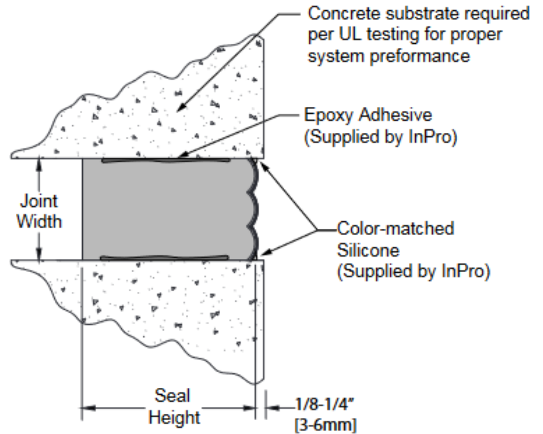
995V3 Series Floor/Floor (995V3-250 System Shown)
